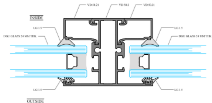
VICO DUAL FIXED GLAZING PLAN
