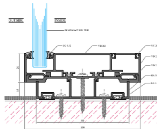
VETRO DUAL FIXED GLAZING SECTION
