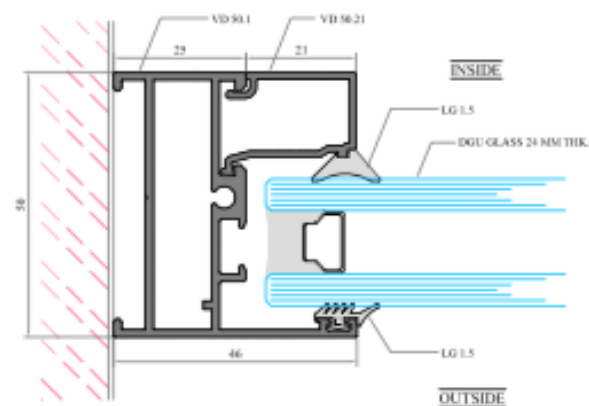
VICO DUAL FIXED GLAZING PLAN
