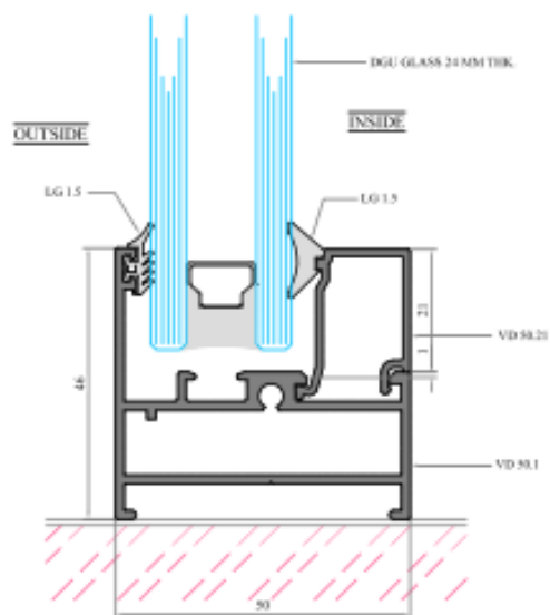
VICO DUAL FIXED GLAZING SECTION
